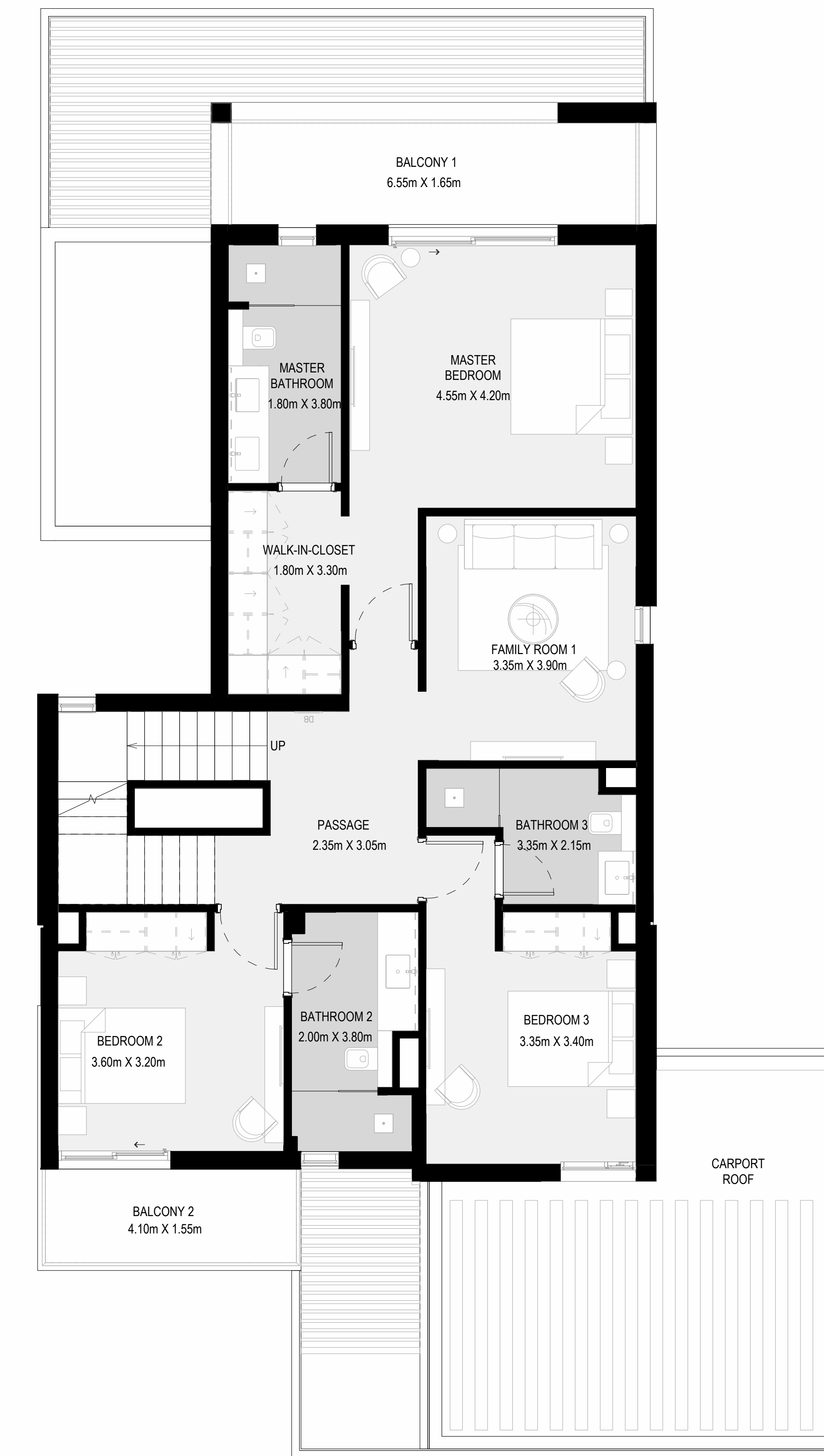
FIRST FLOOR
